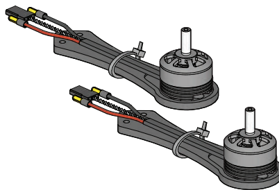
Arm/Motor/ESC Assemblies - CW (Qty 2)
