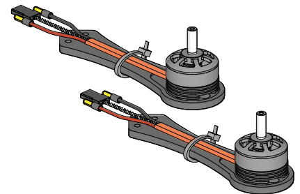
Arm/Motor/ESC Assemblies - CCW (Qty 2)
